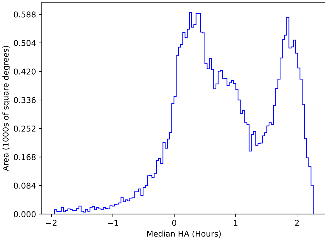
roll_pause_mjdp0_v3.4_10yrs All sky i band: Median HA
