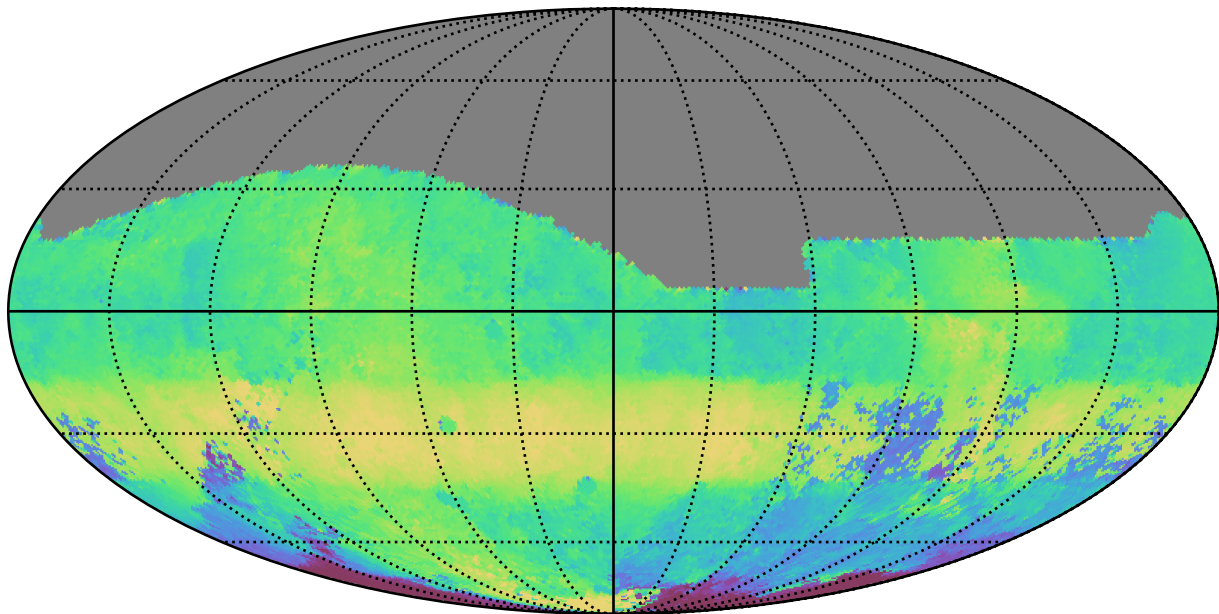
roll_pause_mjdp0_v3.4_10yrs All sky g band: Median HA
