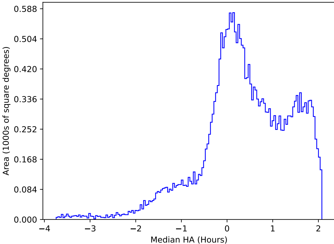
roll_pause_mjdp0_v3.4_10yrs All sky g band: Median HA
