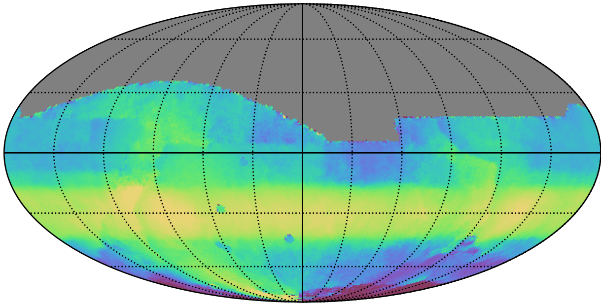
roll_pause_mjdp0_v3.4_10yrs All sky all bands: Median HA
