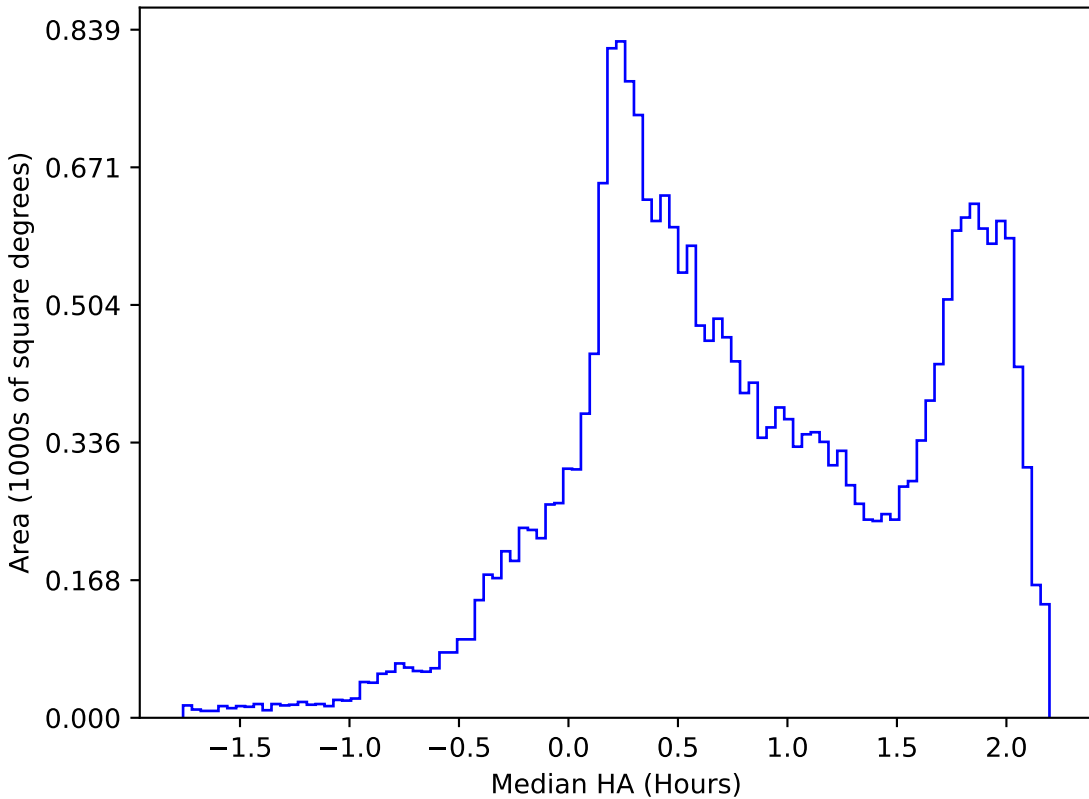
roll_pause_mjdp0_v3.4_10yrs All sky all bands: Median HA
