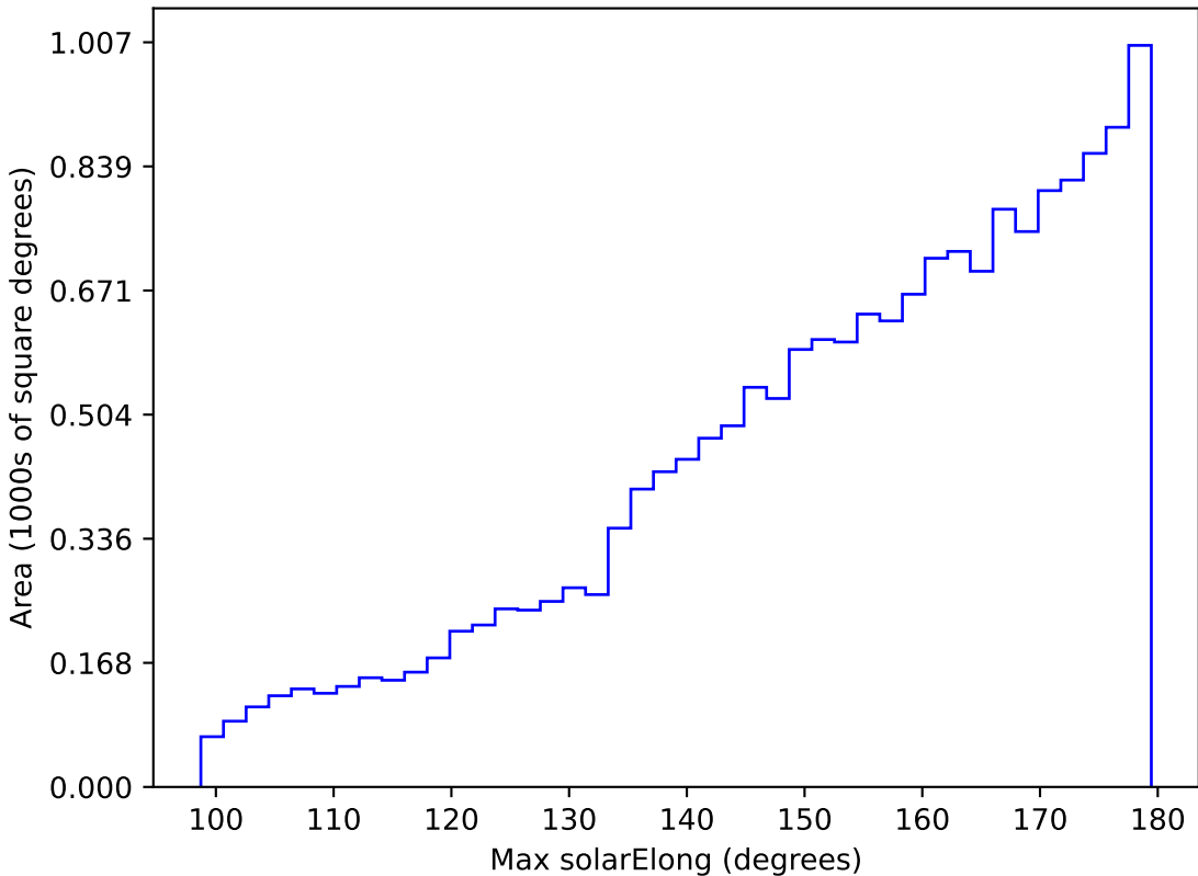
roll_pause_mjdp0_v3.4_10yrs WFD z band: Max solarElong
