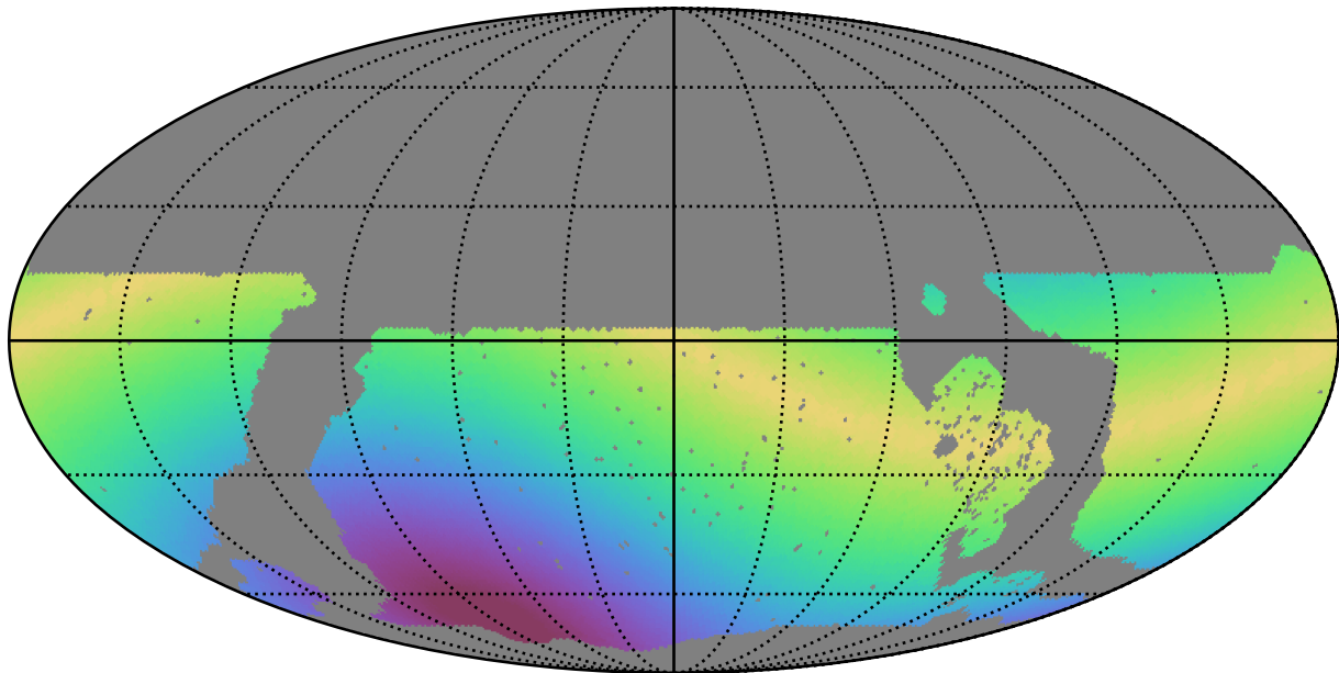
roll_pause_mjdp0_v3.4_10yrs WFD y band: Max solarElong
