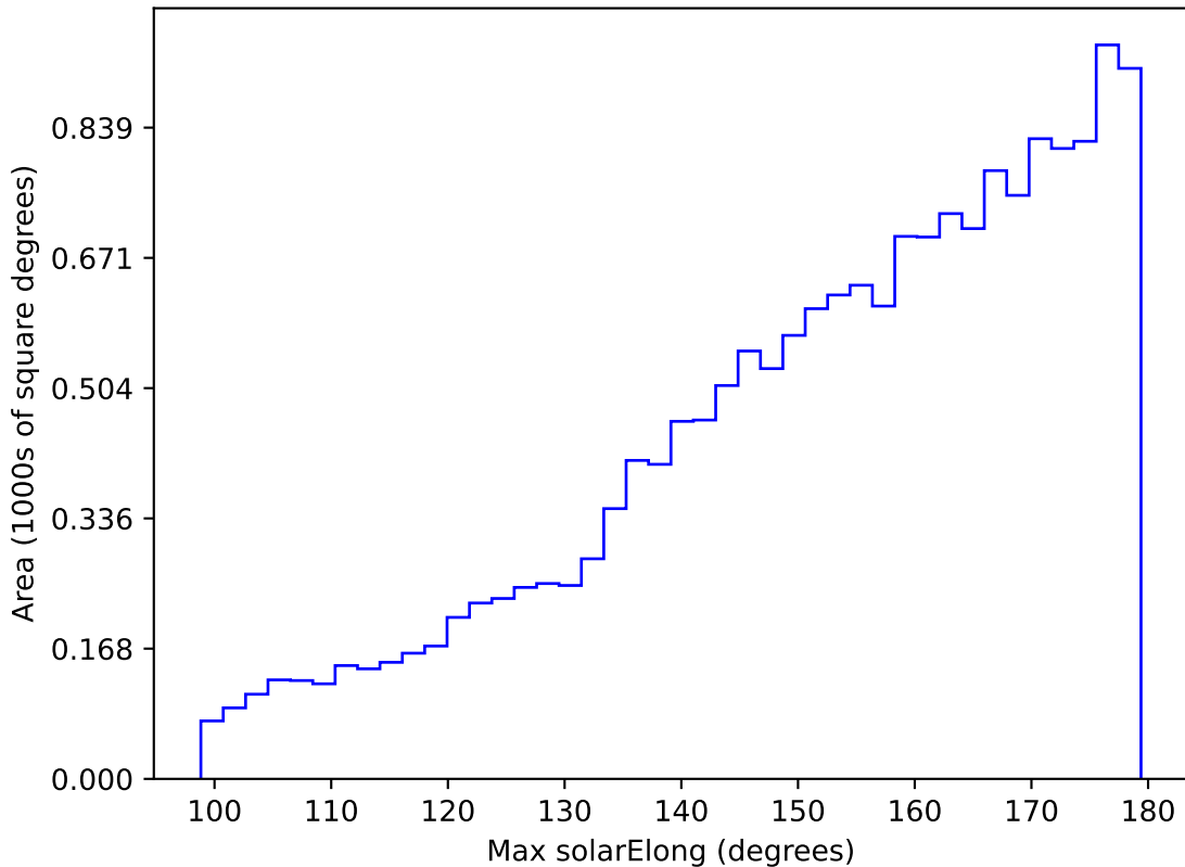
roll_pause_mjdp0_v3.4_10yrs WFD y band: Max solarElong
