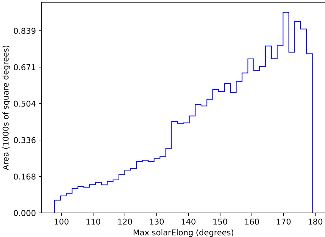
roll_pause_mjdp0_v3.4_10yrs WFD u band: Max solarElong
