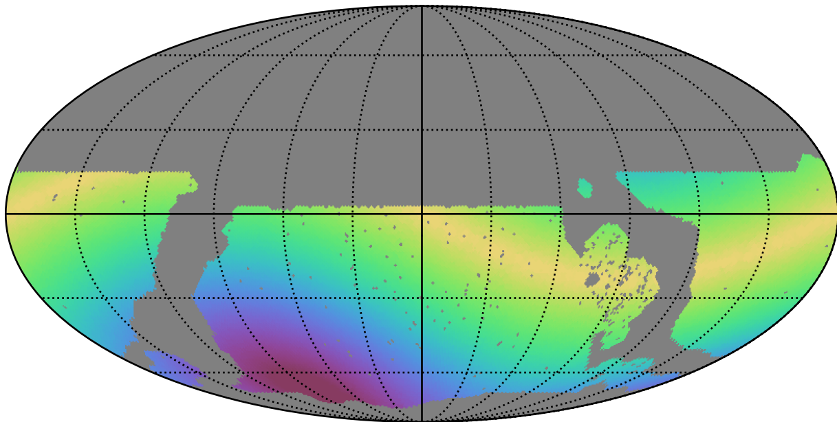
roll_pause_mjdp0_v3.4_10yrs WFD r band: Max solarElong
