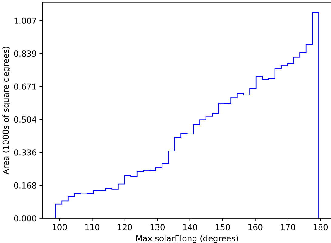
roll_pause_mjdp0_v3.4_10yrs WFD i band: Max solarElong
