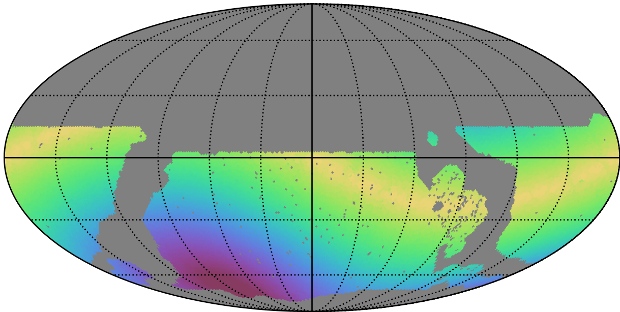
roll_pause_mjdp0_v3.4_10yrs WFD g band: Max solarElong
