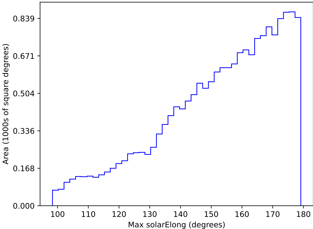
roll_pause_mjdp0_v3.4_10yrs WFD g band: Max solarElong
