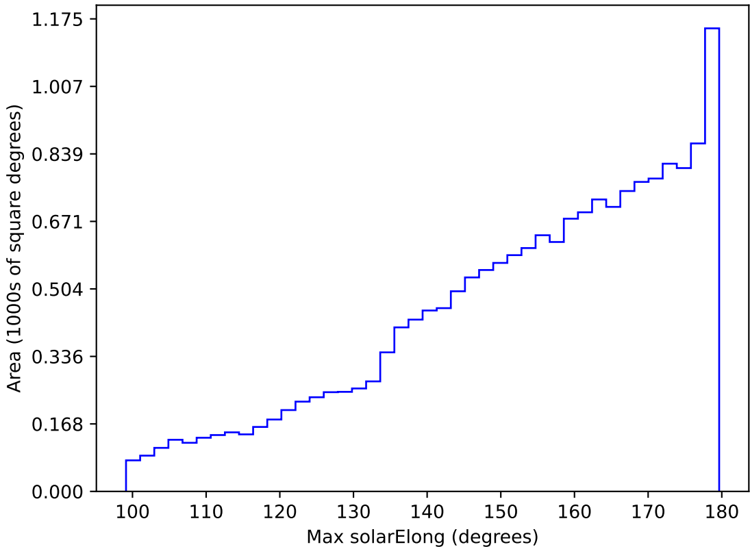
roll_pause_mjdp0_v3.4_10yrs WFD all bands: Max solarElong
