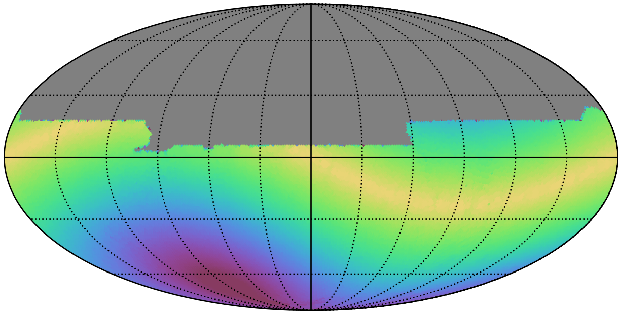
roll_pause_mjdp0_v3.4_10yrs All sky y band: Max solarElong
