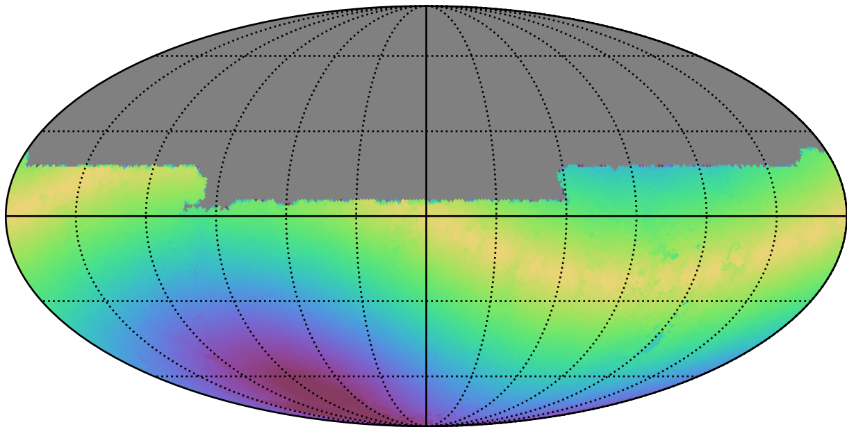
roll_pause_mjdp0_v3.4_10yrs All sky u band: Max solarElong
