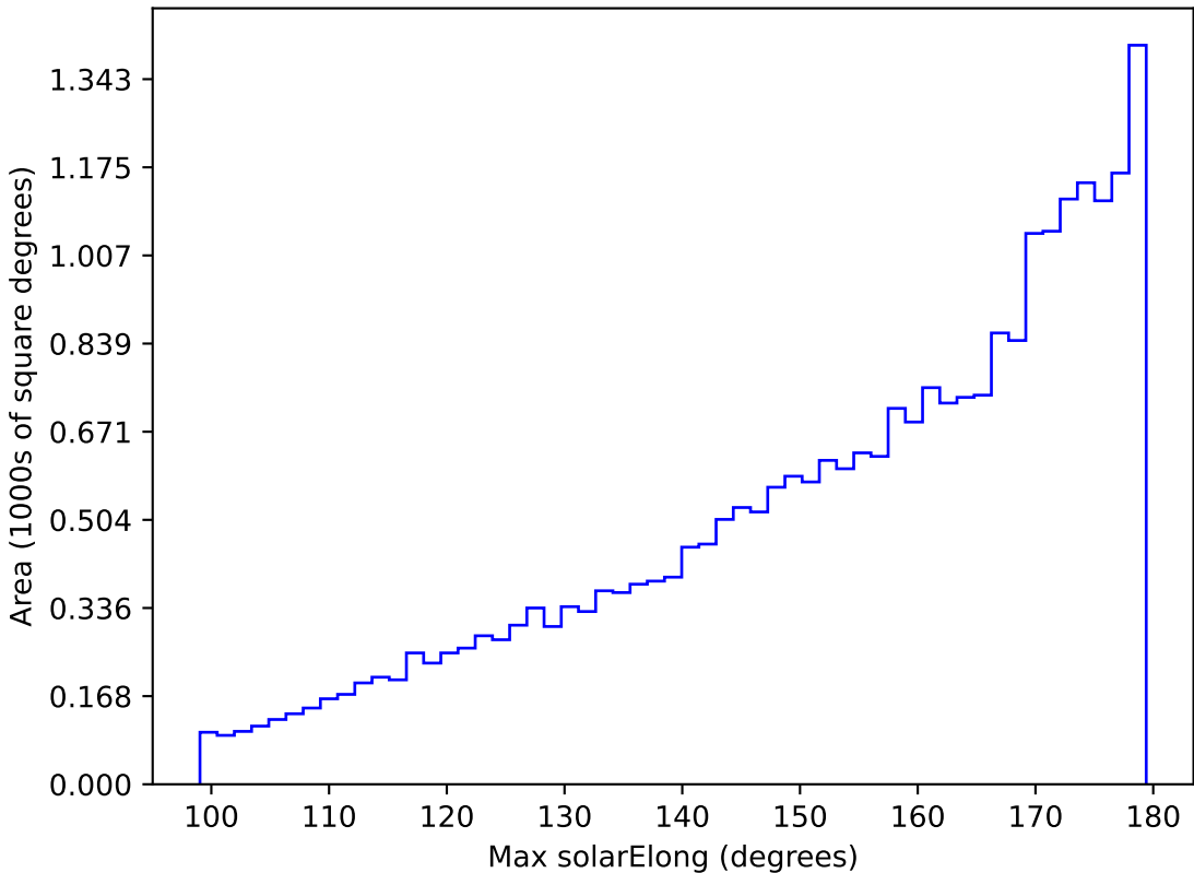
roll_pause_mjdp0_v3.4_10yrs All sky r band: Max solarElong
