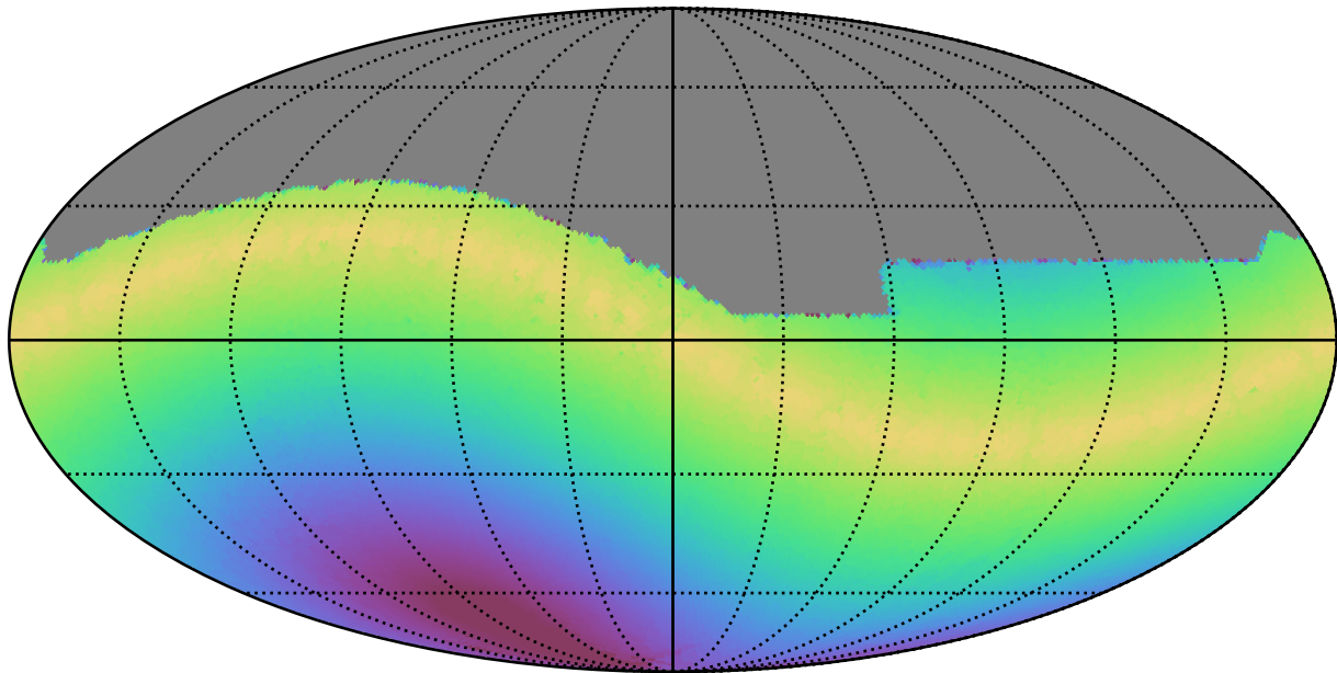
roll_pause_mjdp0_v3.4_10yrs All sky g band: Max solarElong
