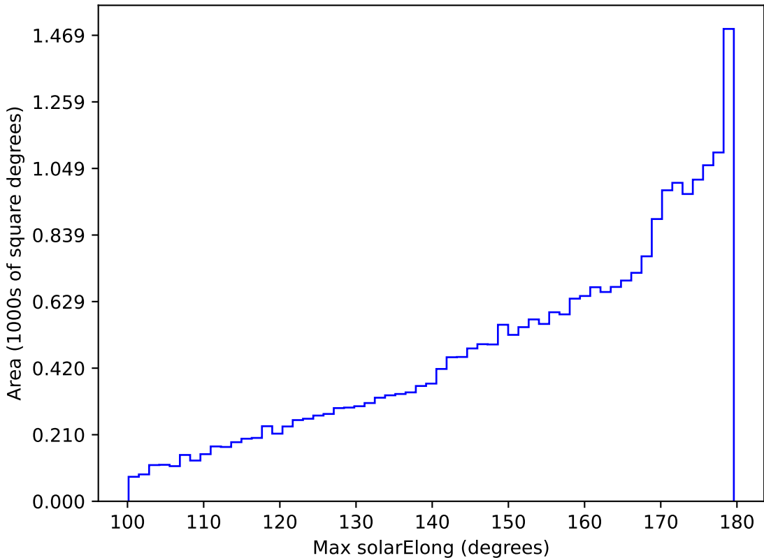
roll_pause_mjdp0_v3.4_10yrs All sky all bands: Max solarElong
