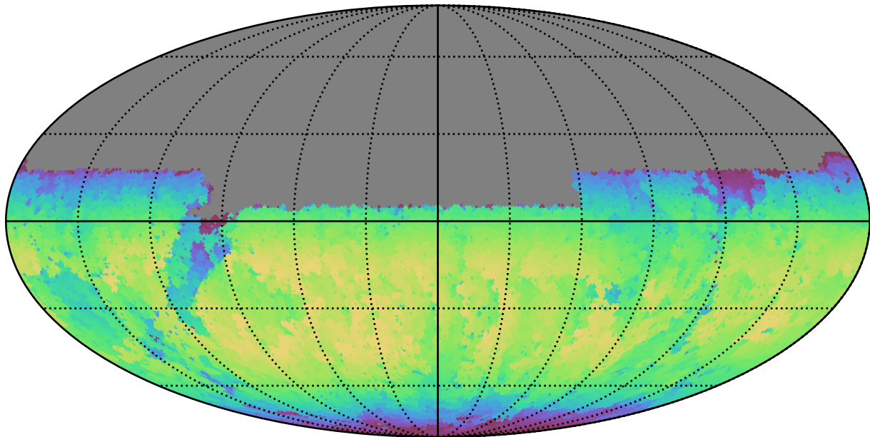
roll_pause_mjdp0_v3.4_10yrs Yr 1 y band: Max skyBrightness
