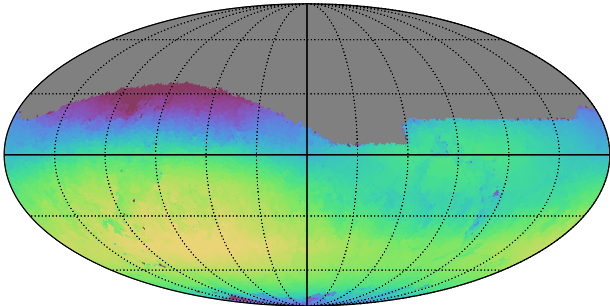
roll_pause_mjdp0_v3.4_10yrs Yr 1 r band: Max skyBrightness
