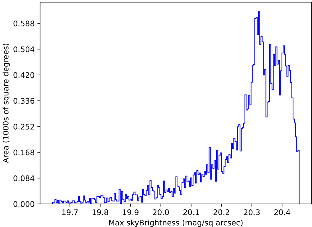
roll_pause_mjdp0_v3.4_10yrs Yr 1 i band: Max skyBrightness
