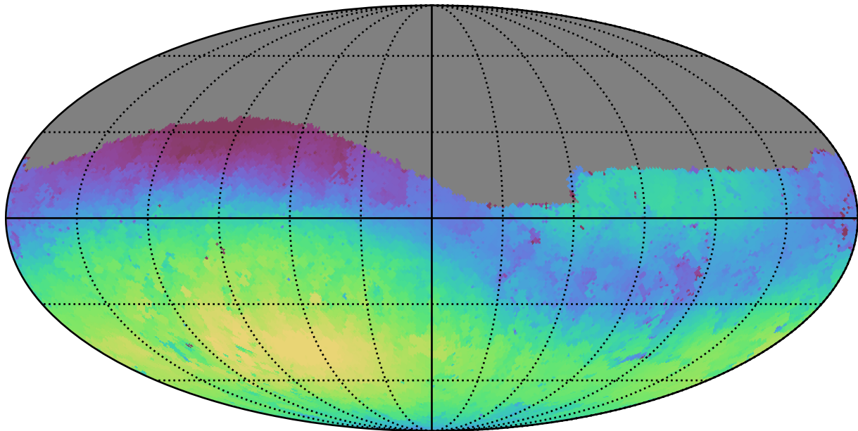
roll_pause_mjdp0_v3.4_10yrs Yr 1 g band: Max skyBrightness
