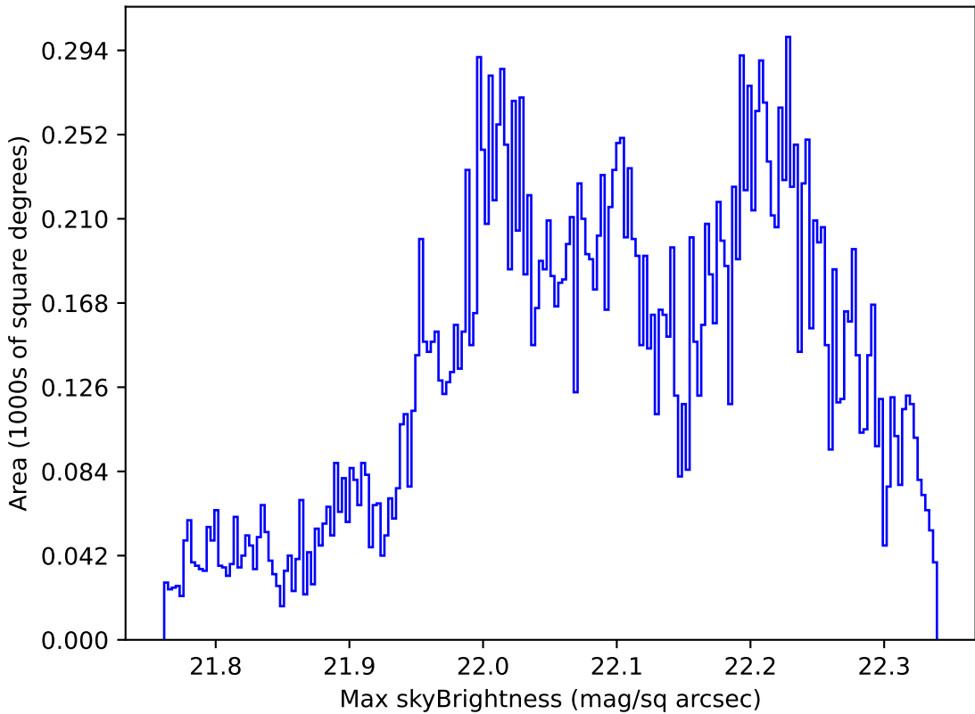
roll_pause_mjdp0_v3.4_10yrs Yr 1 g band: Max skyBrightness
