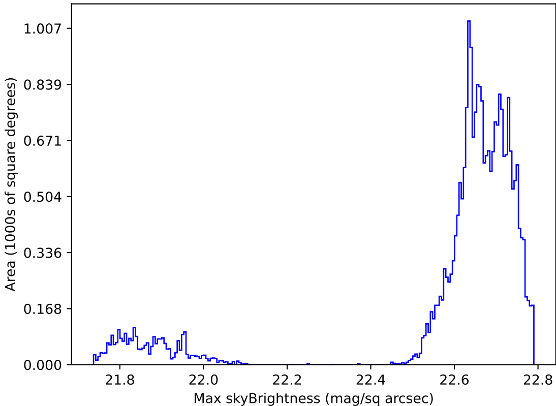
roll_pause_mjdp0_v3.4_10yrs Yr 1 all bands: Max skyBrightness
