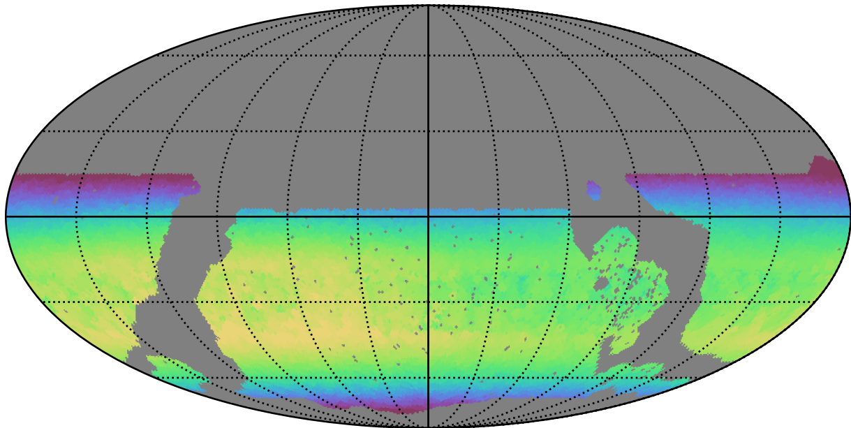
roll_pause_mjdp0_v3.4_10yrs WFD z band: Max skyBrightness
