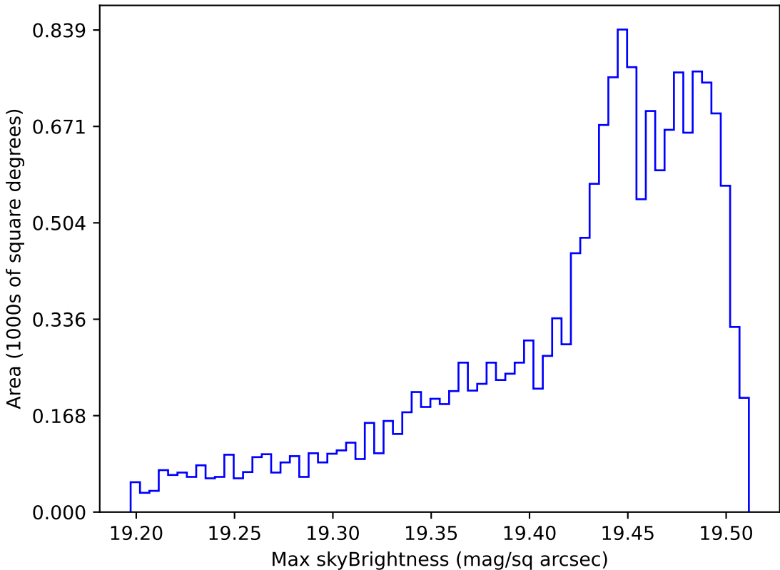
roll_pause_mjdp0_v3.4_10yrs WFD z band: Max skyBrightness
