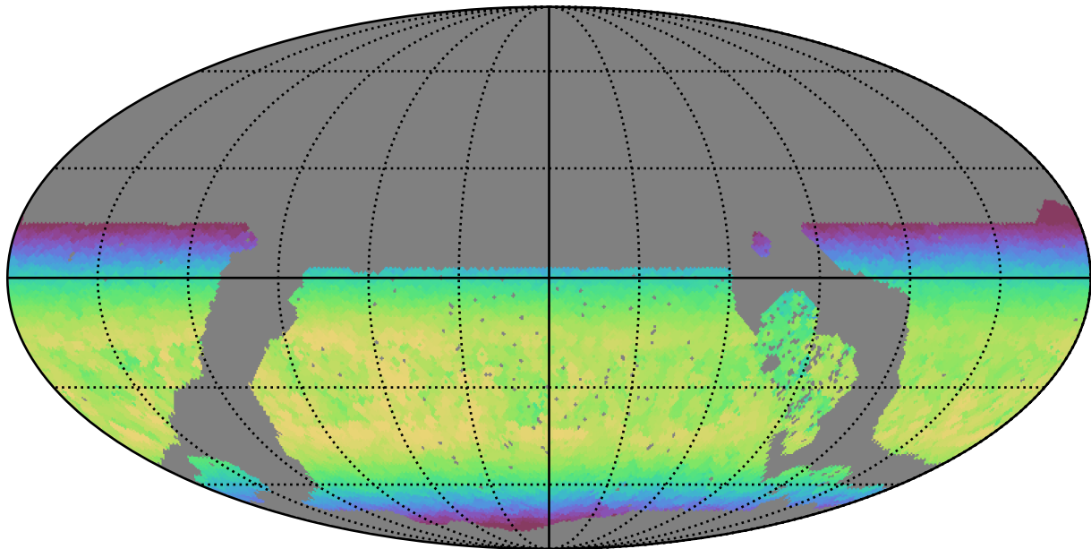
roll_pause_mjdp0_v3.4_10yrs WFD y band: Max skyBrightness
