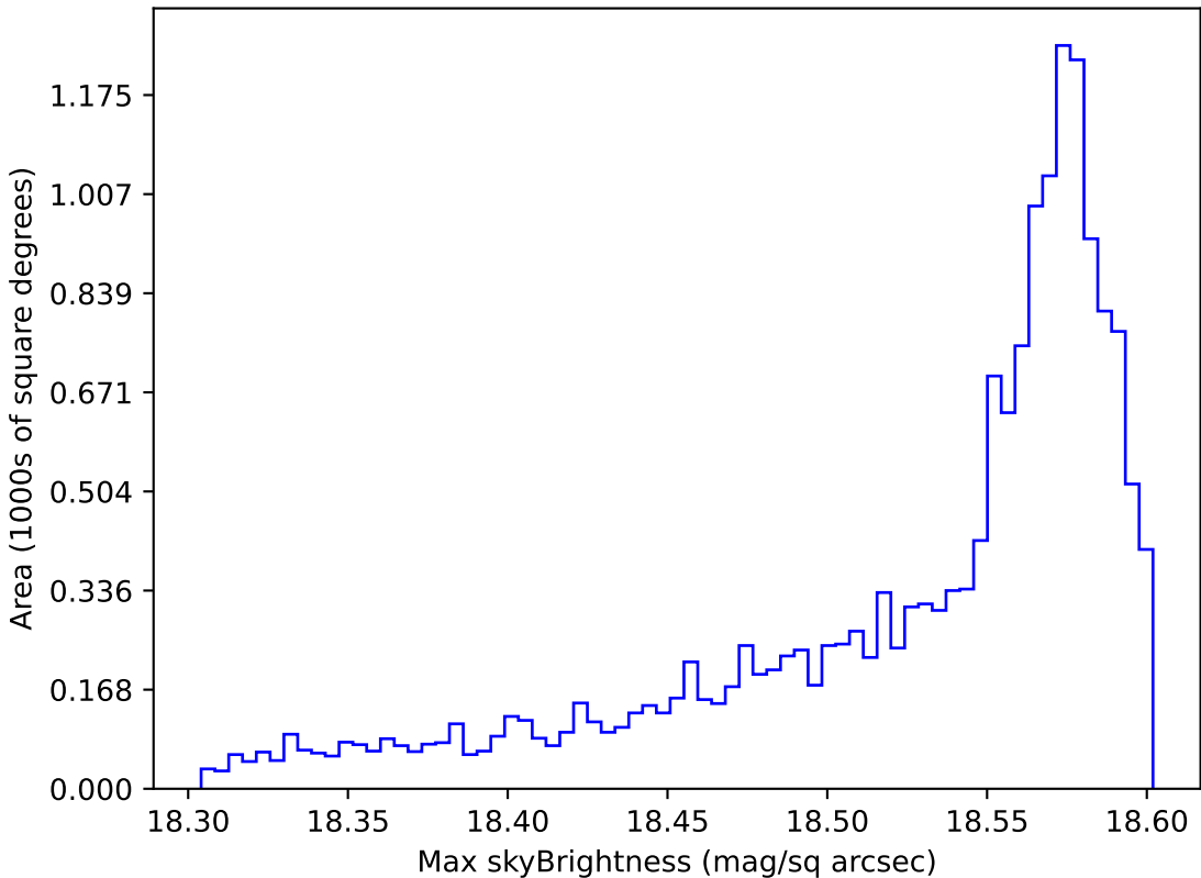
roll_pause_mjdp0_v3.4_10yrs WFD y band: Max skyBrightness
