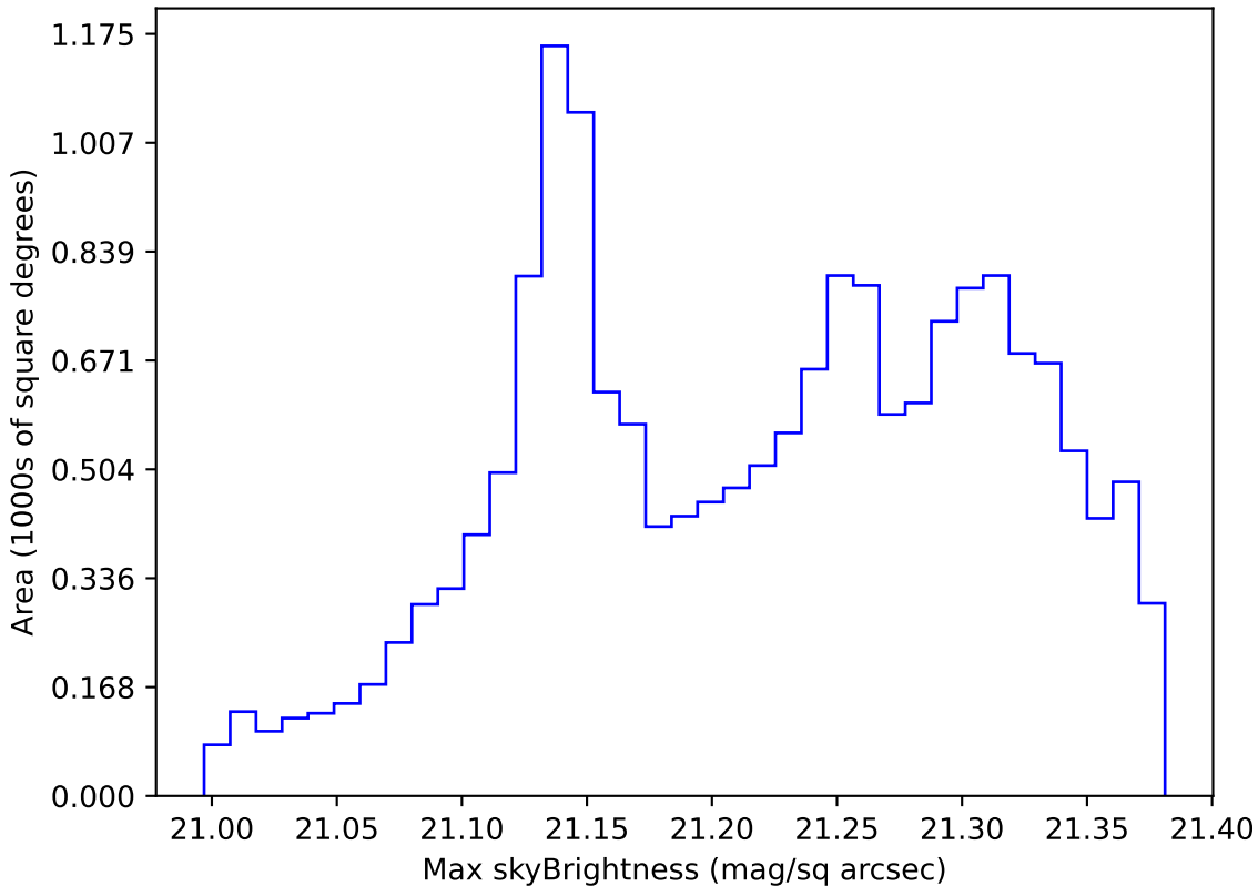
roll_pause_mjdp0_v3.4_10yrs WFD r band: Max skyBrightness
