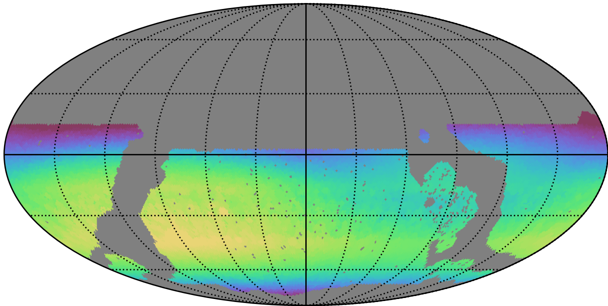
roll_pause_mjdp0_v3.4_10yrs WFD i band: Max skyBrightness
