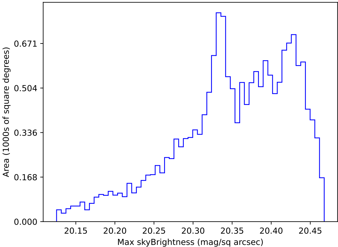
roll_pause_mjdp0_v3.4_10yrs WFD i band: Max skyBrightness
