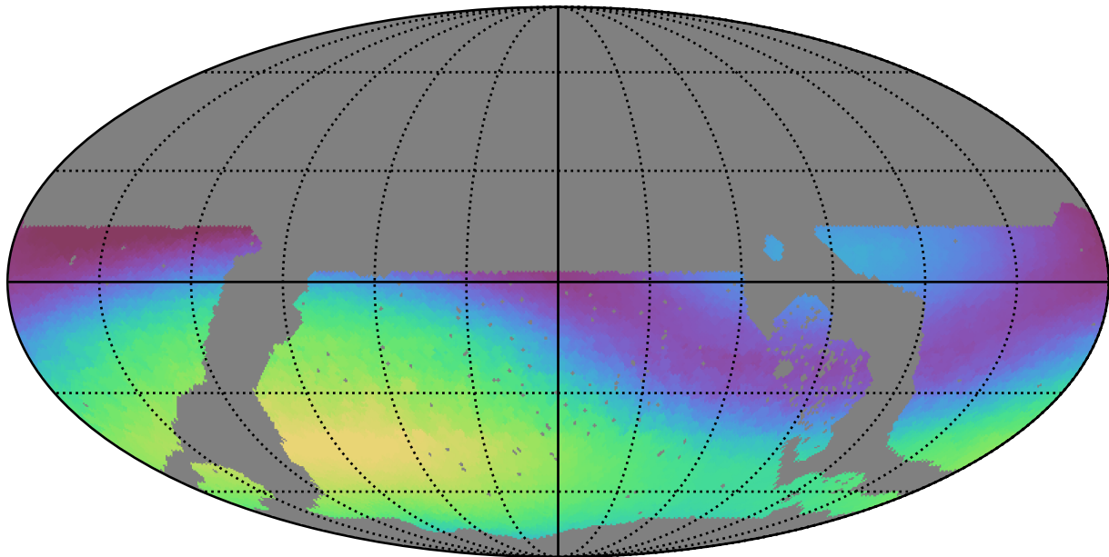
roll_pause_mjdp0_v3.4_10yrs WFD g band: Max skyBrightness
