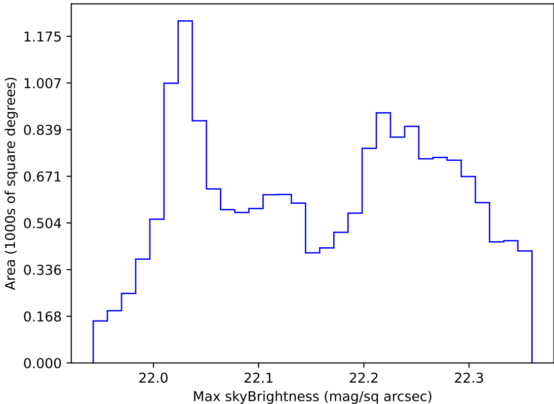
roll_pause_mjdp0_v3.4_10yrs WFD g band: Max skyBrightness
