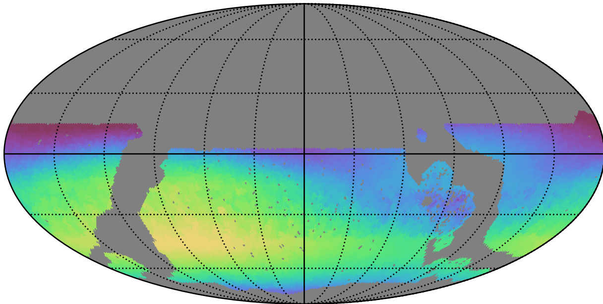
roll_pause_mjdp0_v3.4_10yrs WFD all bands: Max skyBrightness
