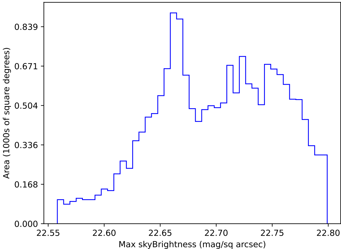
roll_pause_mjdp0_v3.4_10yrs WFD all bands: Max skyBrightness
