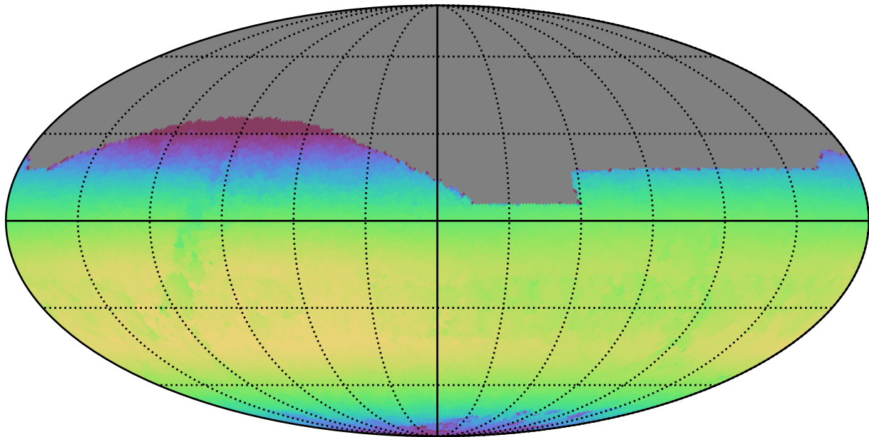
roll_pause_mjdp0_v3.4_10yrs All sky z band: Max skyBrightness
