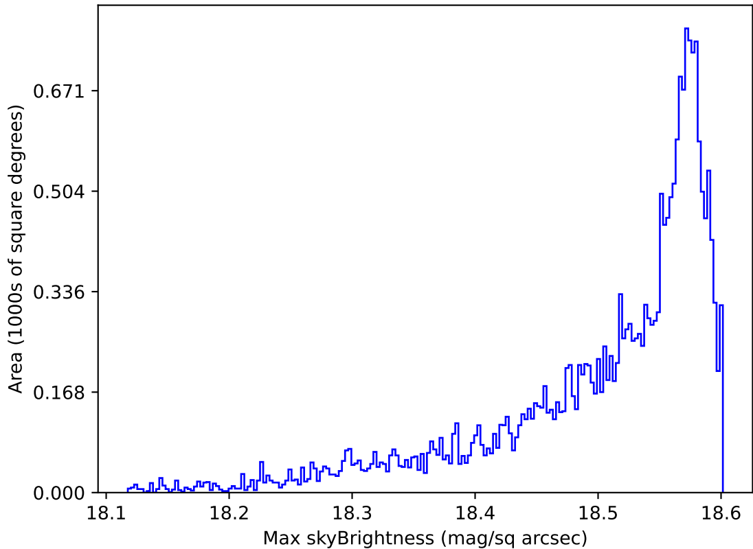
roll_pause_mjdp0_v3.4_10yrs All sky y band: Max skyBrightness
