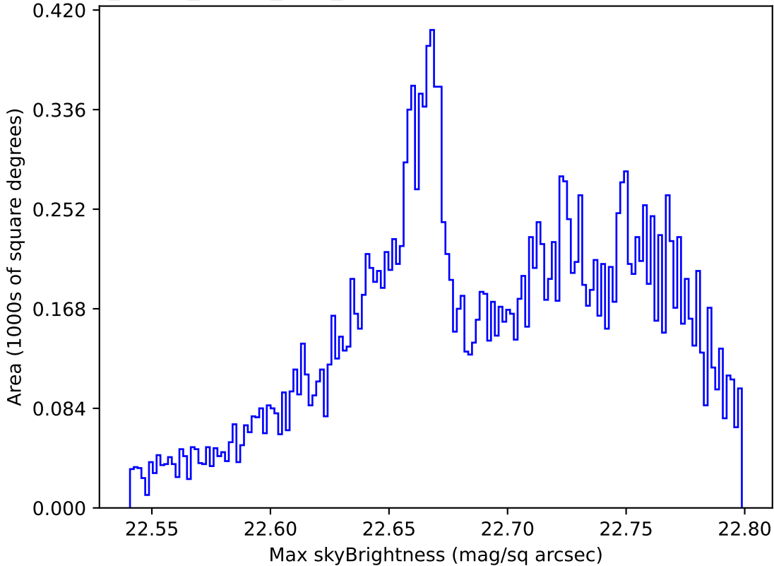
roll_pause_mjdp0_v3.4_10yrs All sky u band: Max skyBrightness
