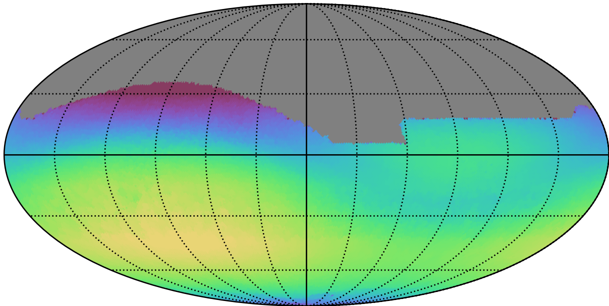
roll_pause_mjdp0_v3.4_10yrs All sky r band: Max skyBrightness
