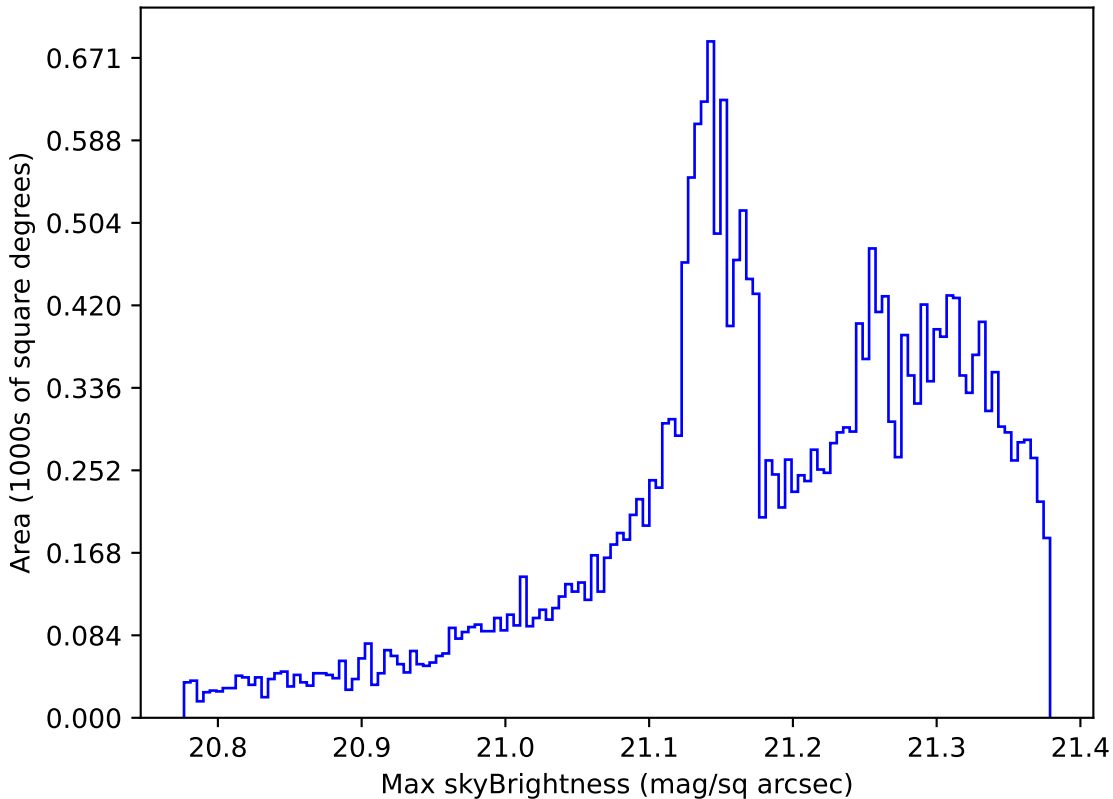
roll_pause_mjdp0_v3.4_10yrs All sky r band: Max skyBrightness
