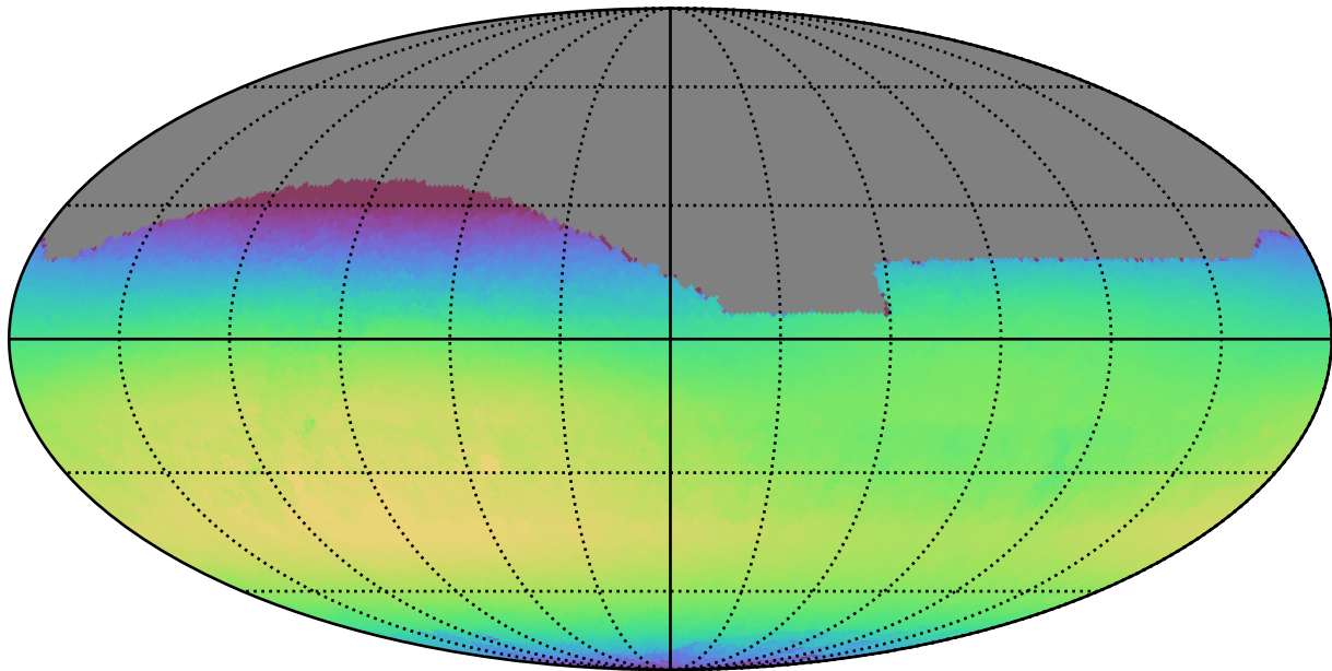
roll_pause_mjdp0_v3.4_10yrs All sky i band: Max skyBrightness
