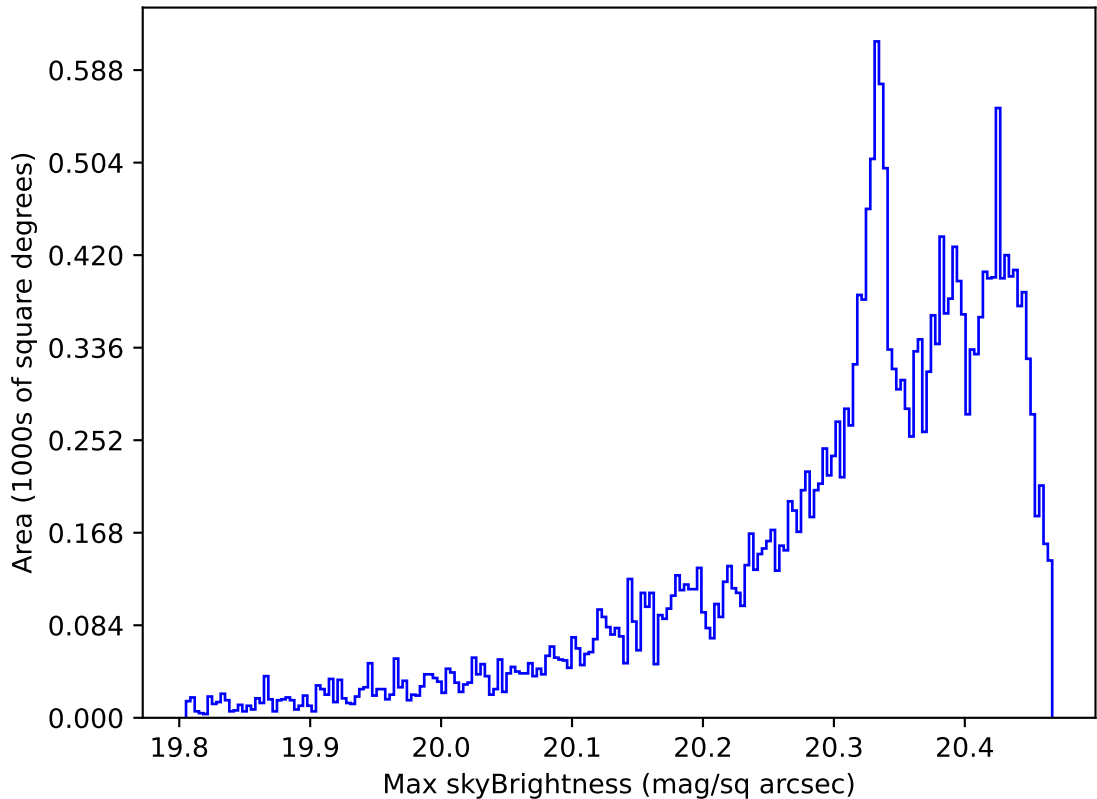
roll_pause_mjdp0_v3.4_10yrs All sky i band: Max skyBrightness
