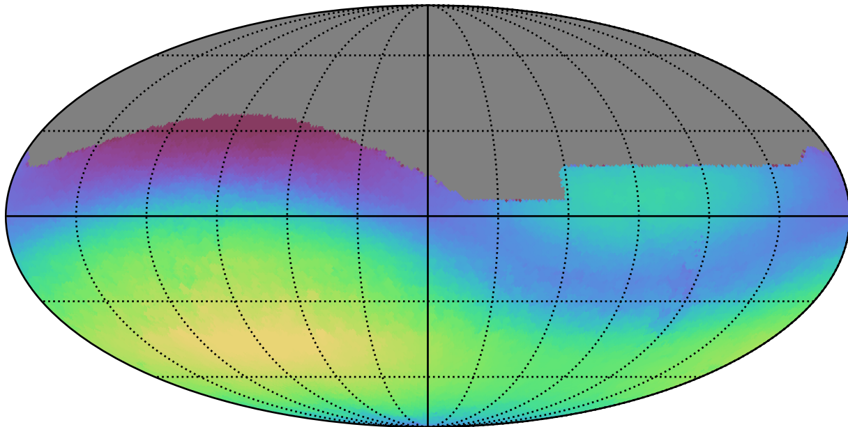
roll_pause_mjdp0_v3.4_10yrs All sky g band: Max skyBrightness
