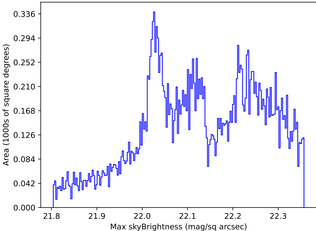
roll_pause_mjdp0_v3.4_10yrs All sky g band: Max skyBrightness
