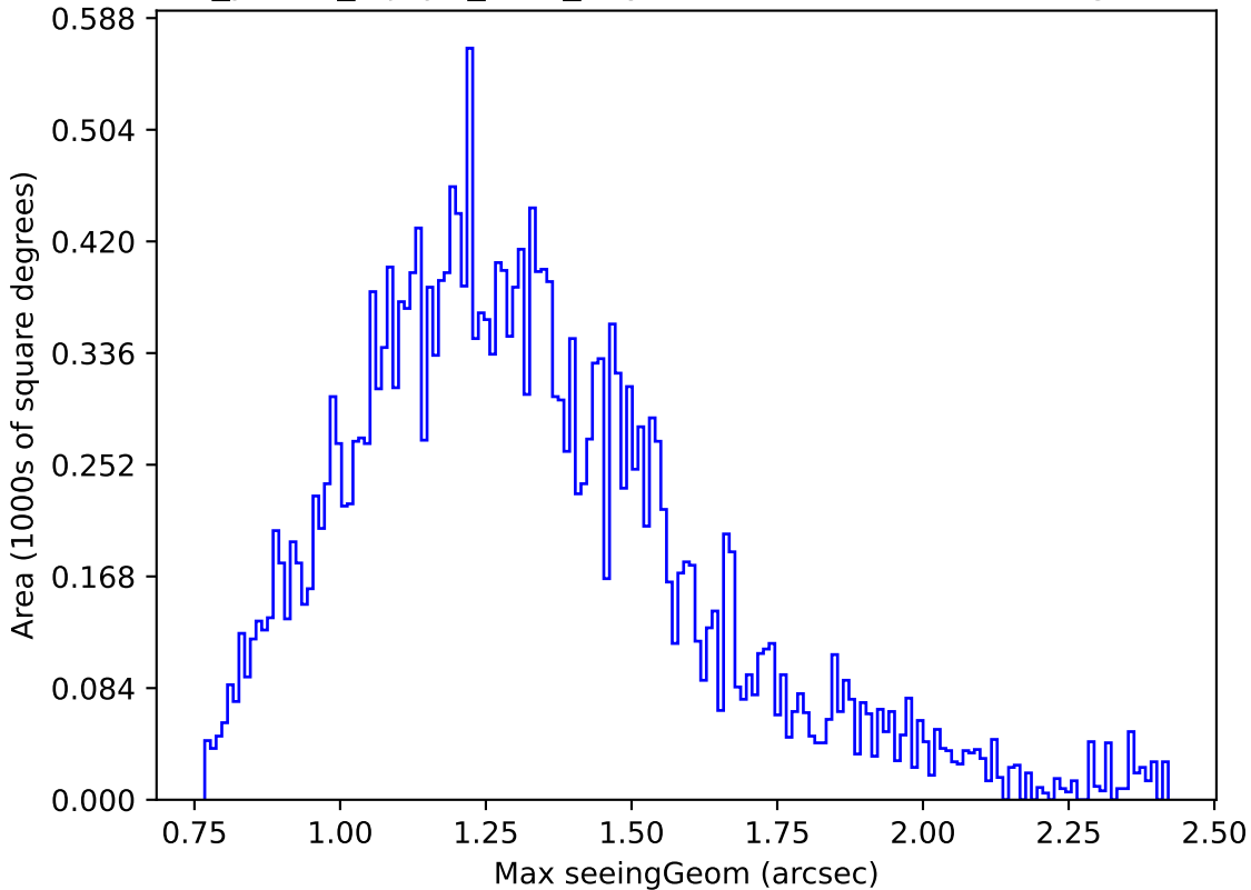
roll_pause_mjdp0_v3.4_10yrs Yr 1 i band: Max seeingGeom
