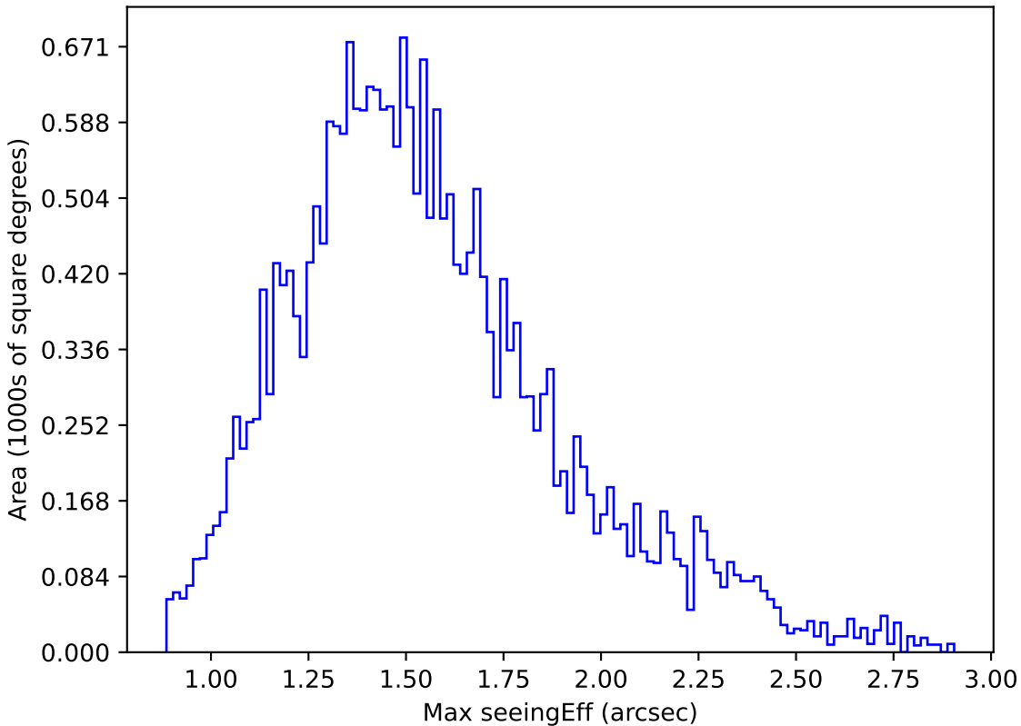
roll_pause_mjdp0_v3.4_10yrs Yr 1 r band: Max seeingEff
