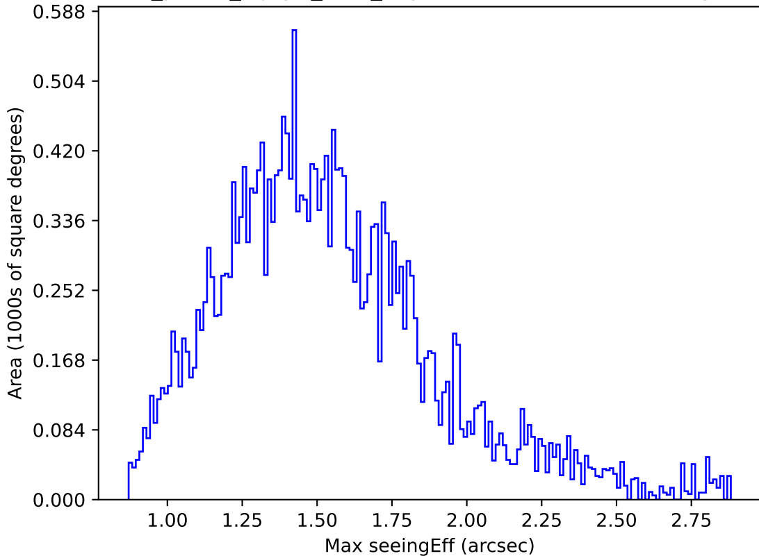
roll_pause_mjdp0_v3.4_10yrs Yr 1 i band: Max seeingEff
