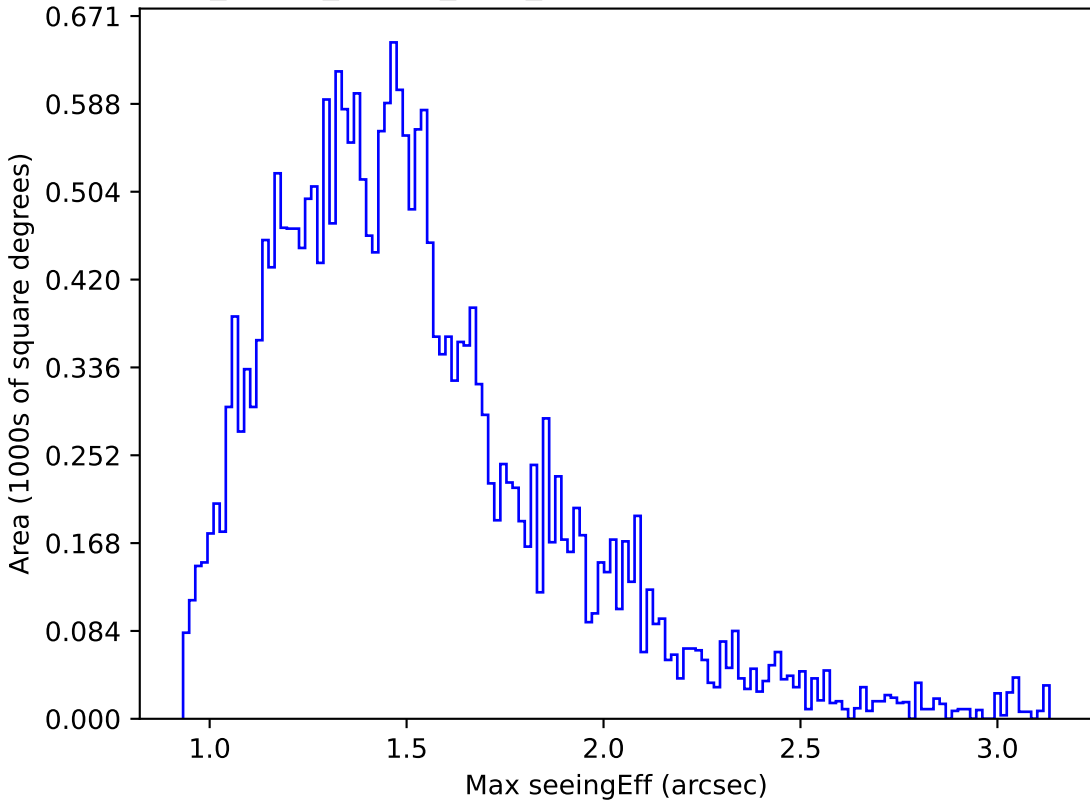
roll_pause_mjdp0_v3.4_10yrs Yr 1 g band: Max seeingEff
