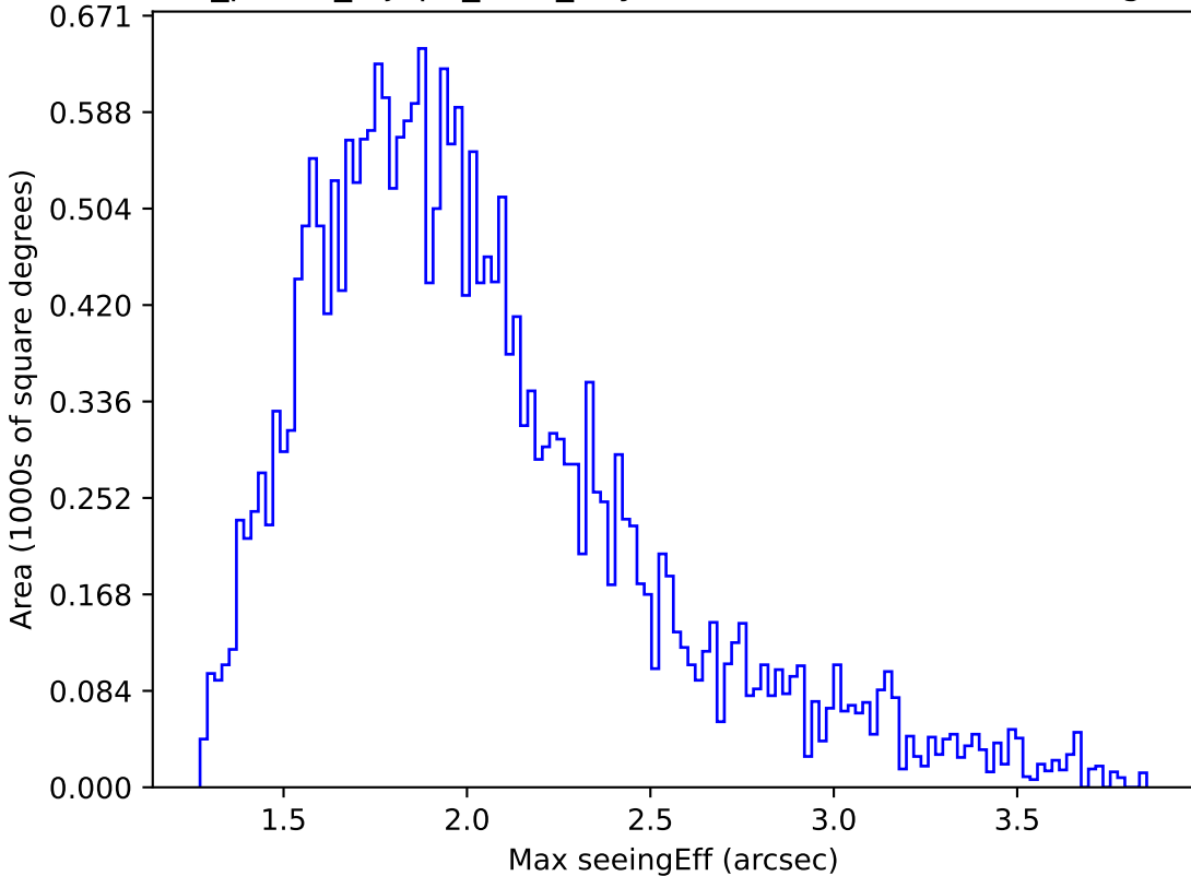
roll_pause_mjdp0_v3.4_10yrs Yr 1 all bands: Max seeingEff
